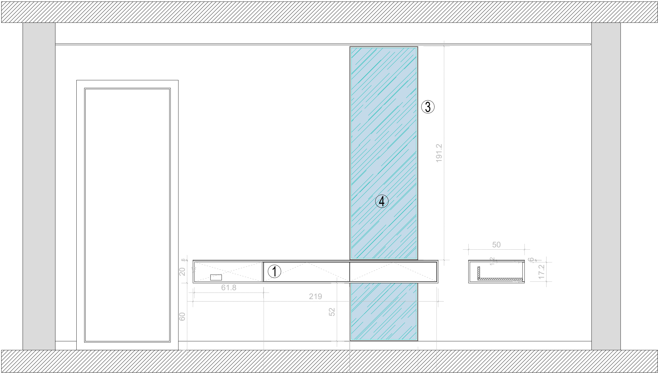
Section Elevation C.C
